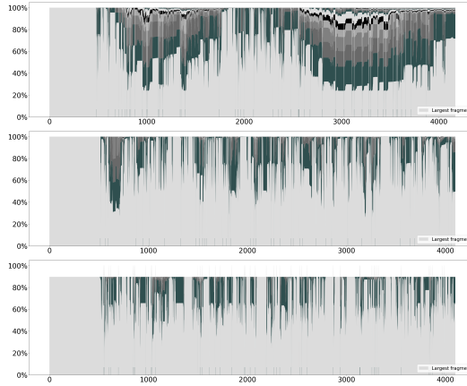
Fig. 9. Fragment adoption during a fragmentation attack, comparing NimbleChain with AT = 4 (top) and AT = 2(C + 1) (middle) against the Ethereum baseline (bottom, no fragmentation attack) The y-axis expresses the percentage of resources owned by each fragment of correct processes, where 100% in the same colour (light grey) means that every correct process' local chain is identical. The x-axis represents time, in seconds.
